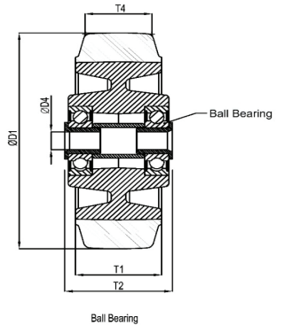
Ball Bearing
