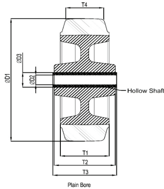
Plain Bore
