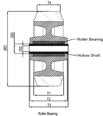
Roller Bearing
