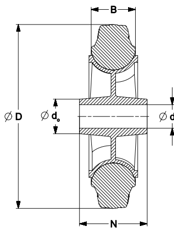
Plain Bearing
