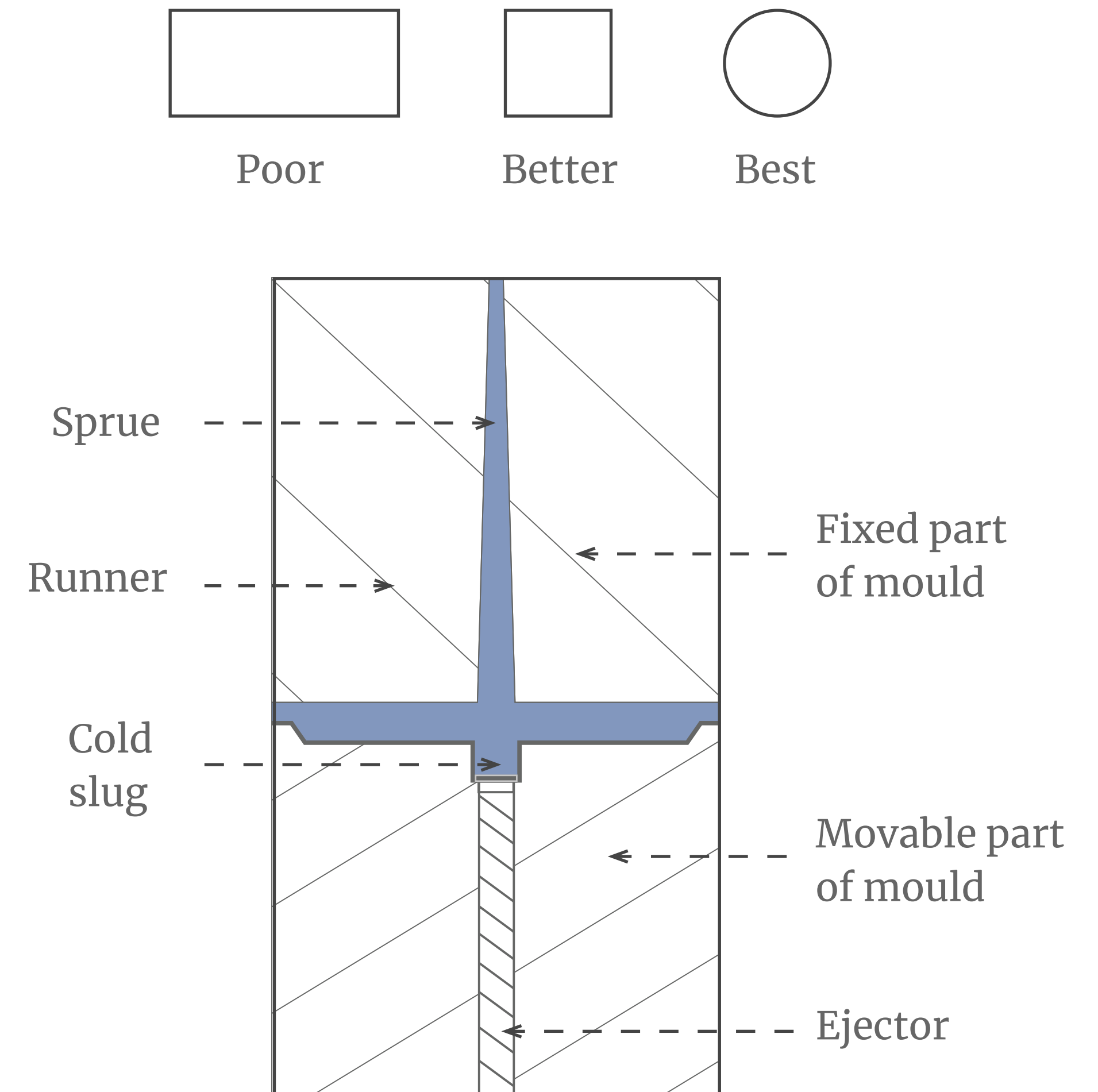
Figure 2 : Cold Slug
