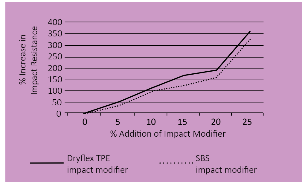
FIGURE 2. INCREASE IN IMPACT RESISTANCE OF POLYSTYRENE REGRIND
