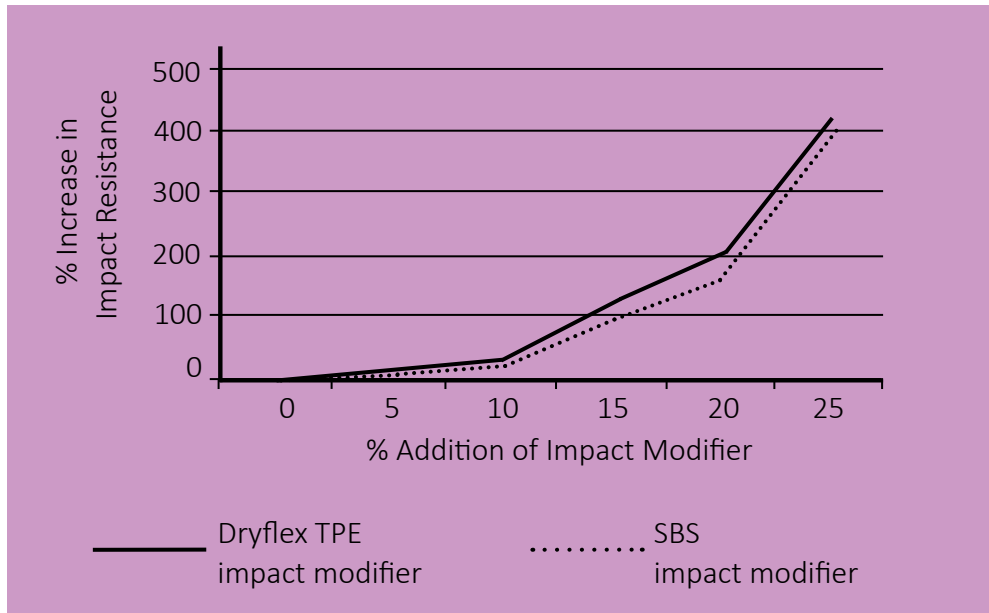
FIGURE 1. INCREASE IN IMPACT RESISTANCE OF VIRGIN CRYSTAL POLYSTYRENE
